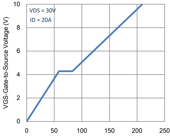
7. Gate Charge
