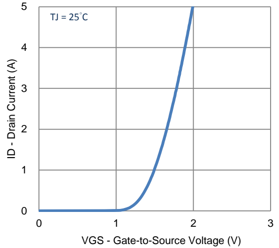
2. Transfer Characteristics
